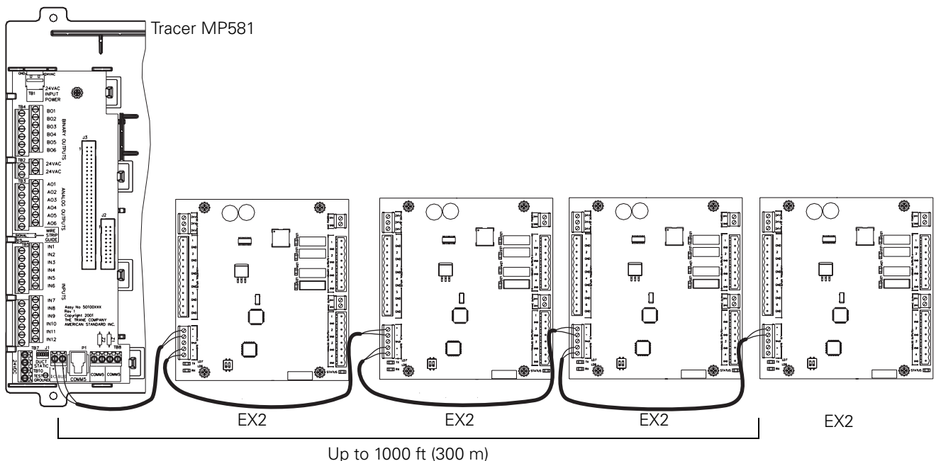
Figure 48. I/O bus wiring example 1
